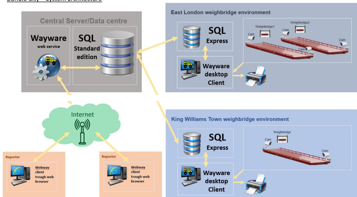
Buffalo City – System architecture
